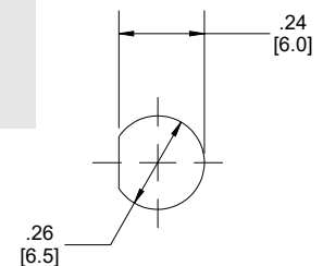
MOUNTING HOLE
