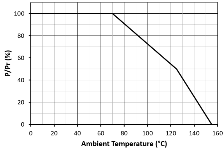
Temperature Derating
