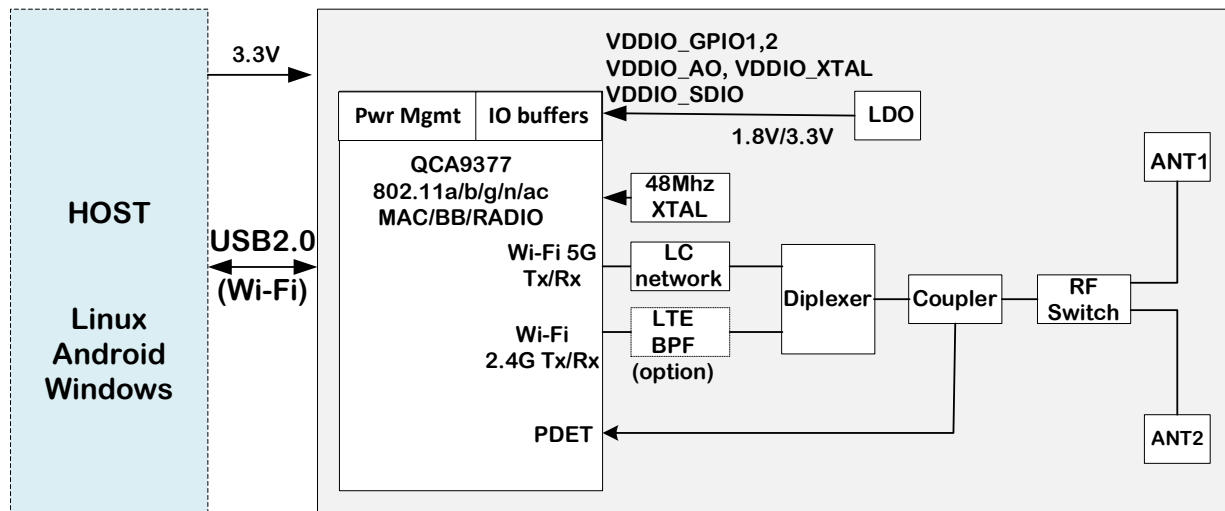
Figure 1: EVIA M.2 USB Block Diagram
