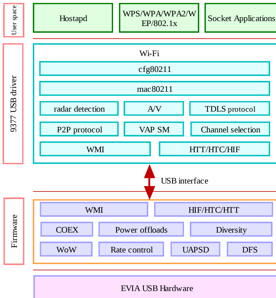
Figure 2: EVIA M.2 Software Architecture
