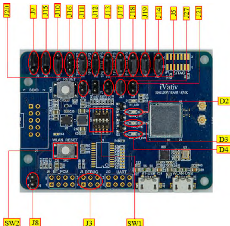
Figure 1: EVIA USB EVK
