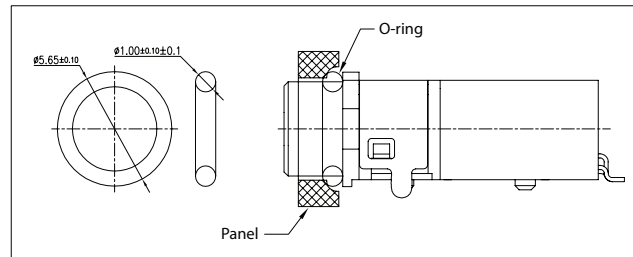
O-Ring Assembly
