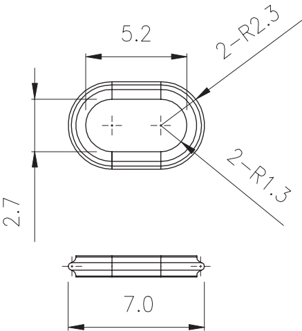
O-ring (P/N: OR-60)
