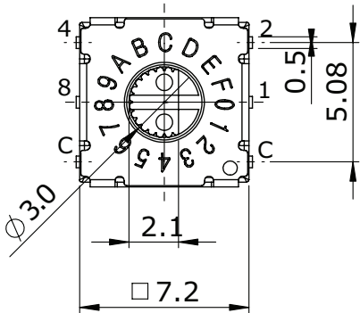
16 POSITION
