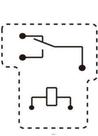
Wiring Diagram Bottom View
