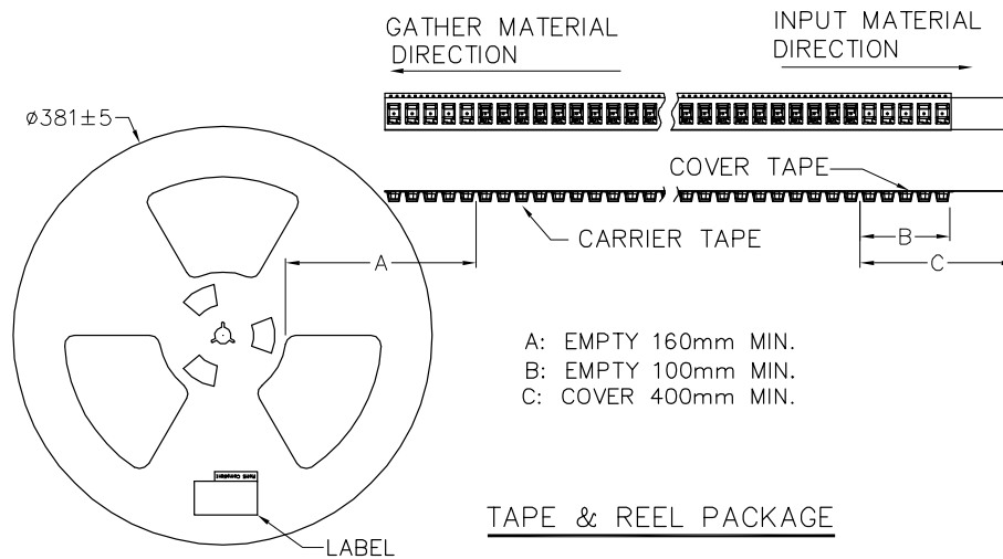
CARRIER TAPE
