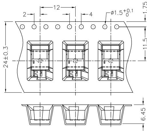
CARRIER TAPE
