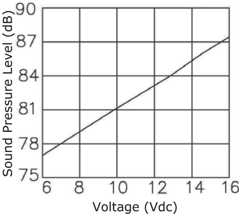
Voltage vs. Sound Pressure Level at 60 cm
