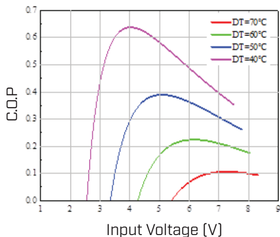
COP Vs. Input Voltage, V ( \Delta T=40\sim 70^\circ C )
