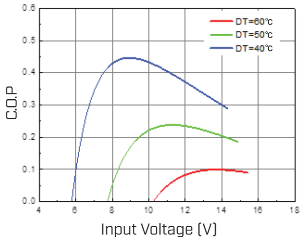
COP Vs. Input Voltage, V ( \Delta T=40\sim60^{\circ}C )
