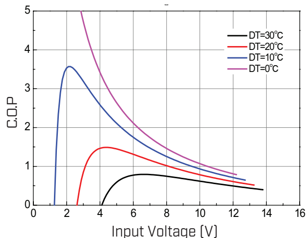
COP Vs. Input Voltage, V ( \Delta T=0\sim30^{\circ}C )
