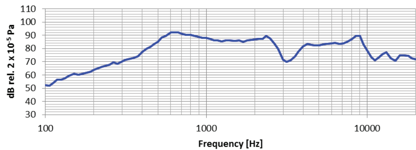
Frequency Response Curve
