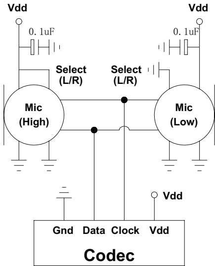
Dual Microphone
