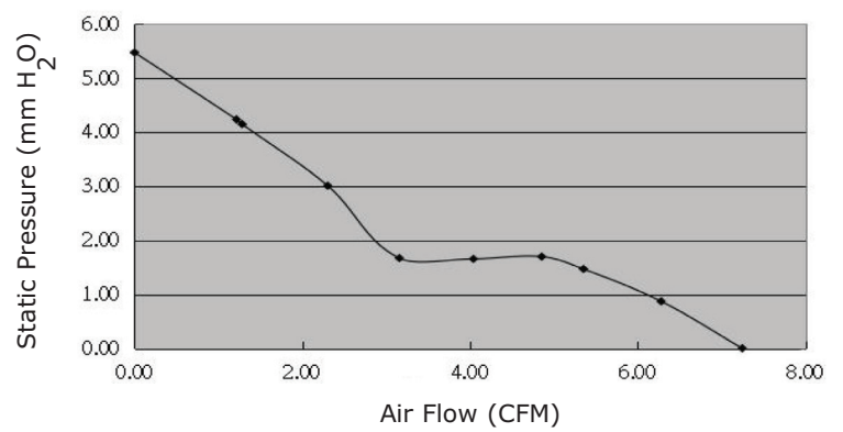
CFM-4015C-265-256
