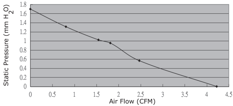
CFM-4010C-050-195
