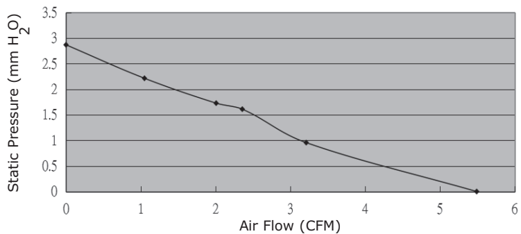
CFM-4010C-165-251
