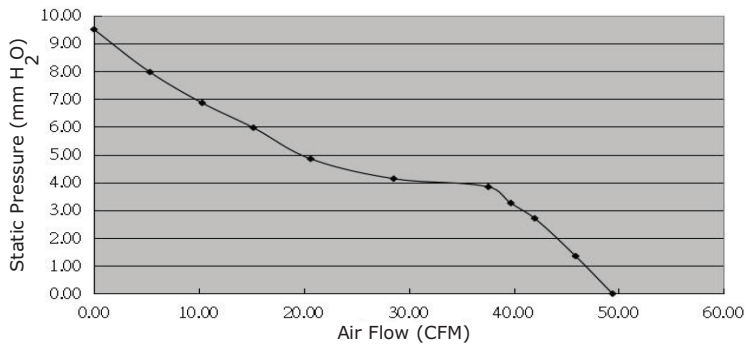
CFM-8038B-140-449
