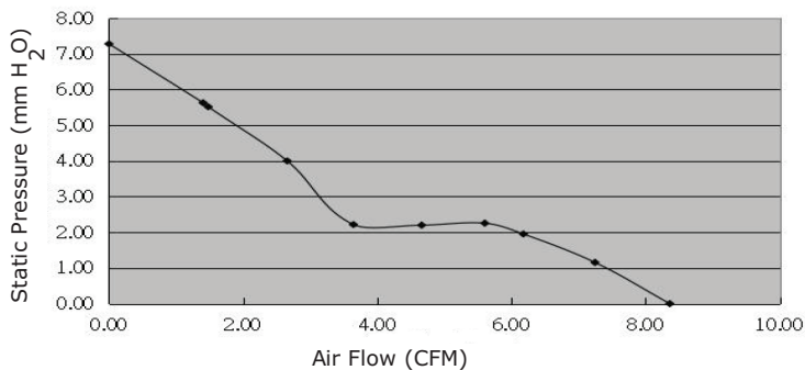
CFM-4015C-175-287
