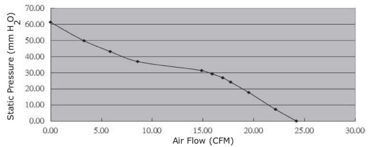
CFM-4028BG-1200-568
