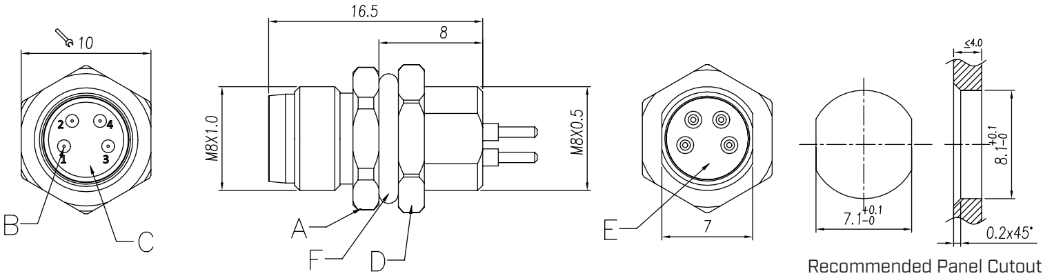
Recommended Panel Cutout
