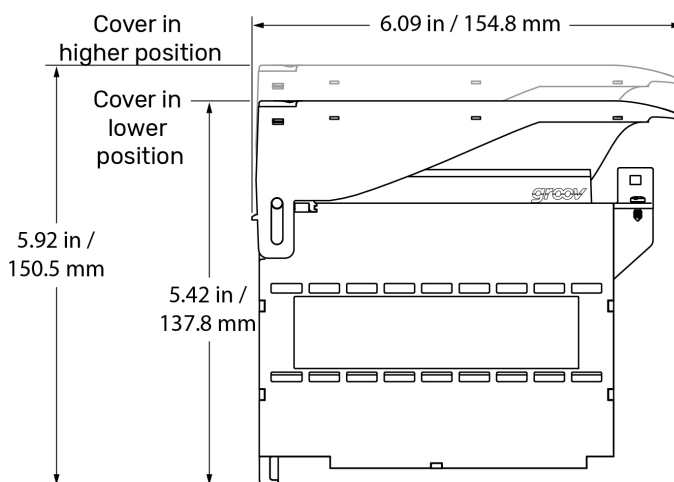
GRV-IACDCTTL-24, GRV-IACDCTTLS-24
