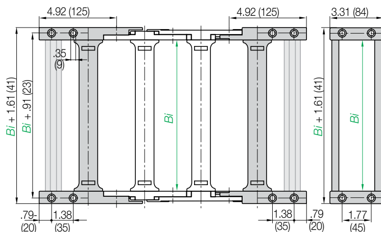
Fixed end E4-561...2
