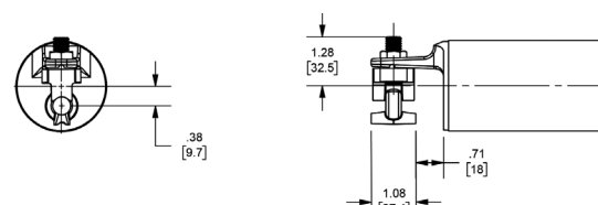
Fig. 2. Eyebolt only, for 6-2/O cable (9F59AAW008)
