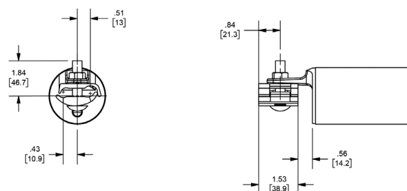
Fig. 3. Parallel groove only, for 2/O to 250MCM cable (9F59AAW009)
