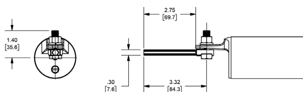
Fig. 1. Adapter only (9F59AAW007)
