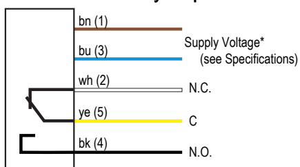
Electromechanical Relay Output Models
