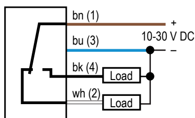
PNP (Sourcing) Solid-State Output Models
