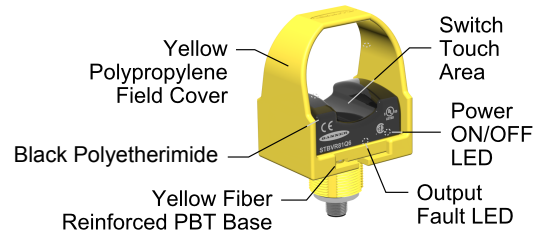
STB Touch Button features
