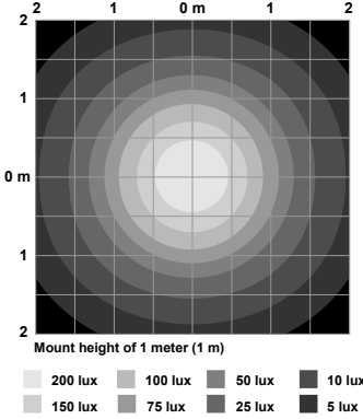
Isolux Pattern
