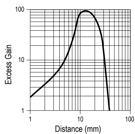
Excess Gain Curve with 40 mm Cutoff (based on 90% White Card)
