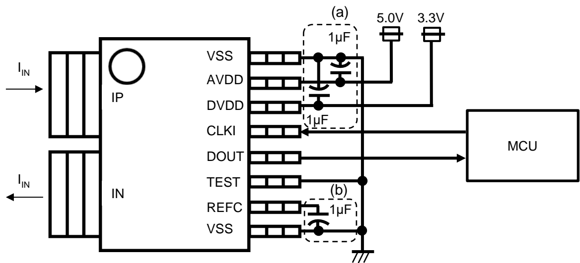
Figure 7. Recommend External Circuit of CQ-363x
