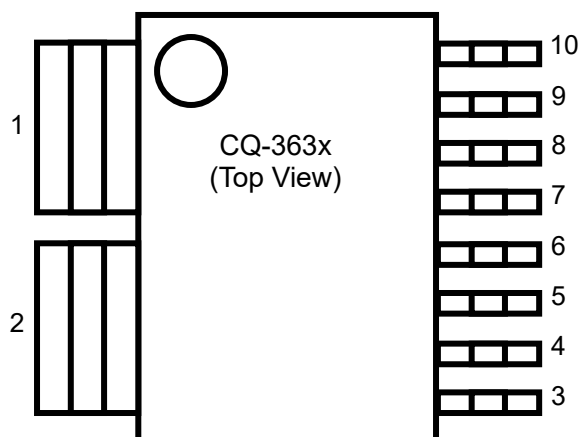
Figure 2. Pin configurations of CQ-363x
