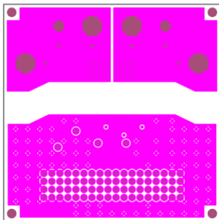
Figure 8. Board layout for measuring thermal resistance of CQ-363x
