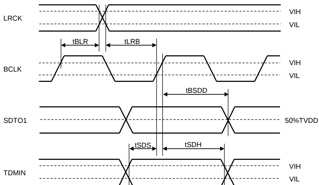
Figure 8. Audio Interface Timing (TDM &amp; Slave mode: BCKP bit = "0")
