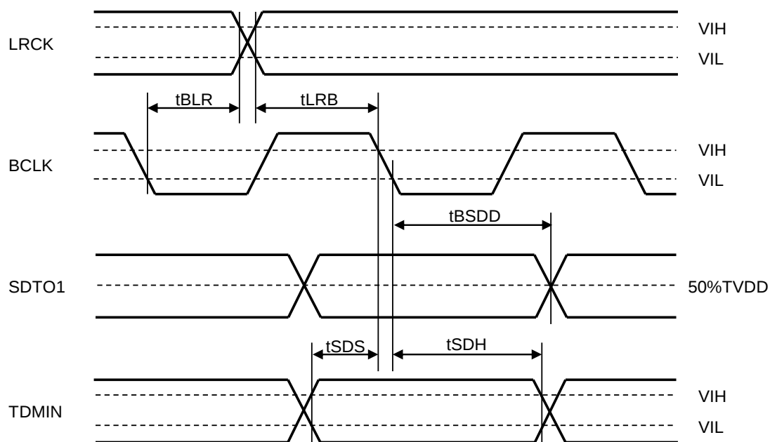
Figure 9. Audio Interface Timing (TDM &amp; Slave Mode: BCKP bit = "1")
