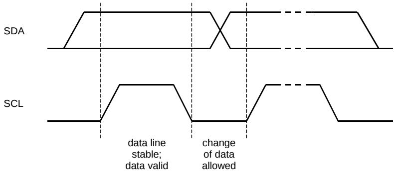
Figure 55. Bit Transfer (I²C Bus)
