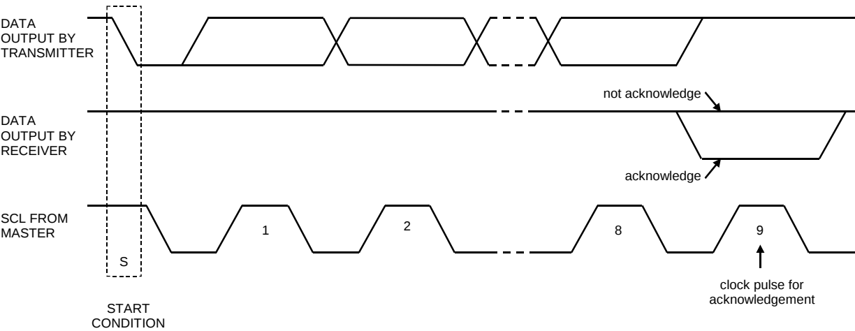
Figure 54. Acknowledge (I²C Bus)
