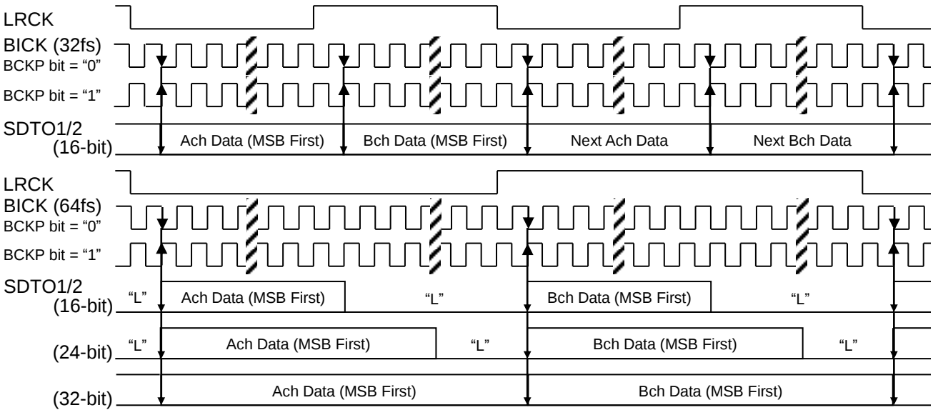
Figure 18. Mode 0/4 Timing (Normal mode, I²S Compatible)
