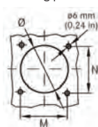
drilling pattern
