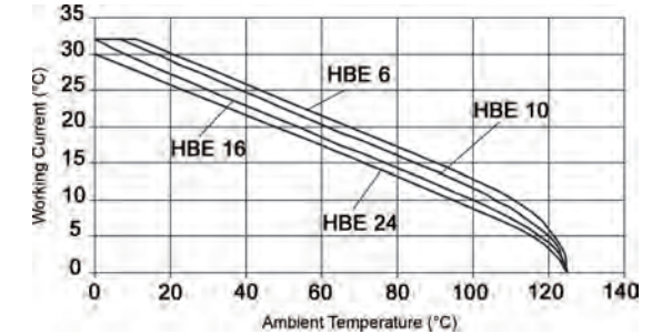
14 AWG (2.5 mm²) crimp termination
