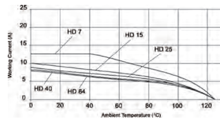
14 AWG (2.5 mm 2 ) machined contacts
