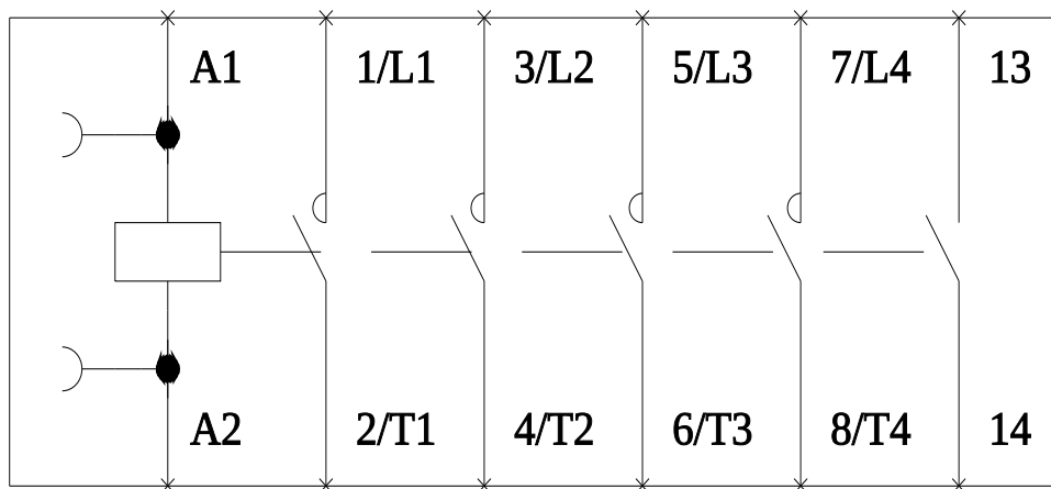
LEN00B004 Wiring Diagram
