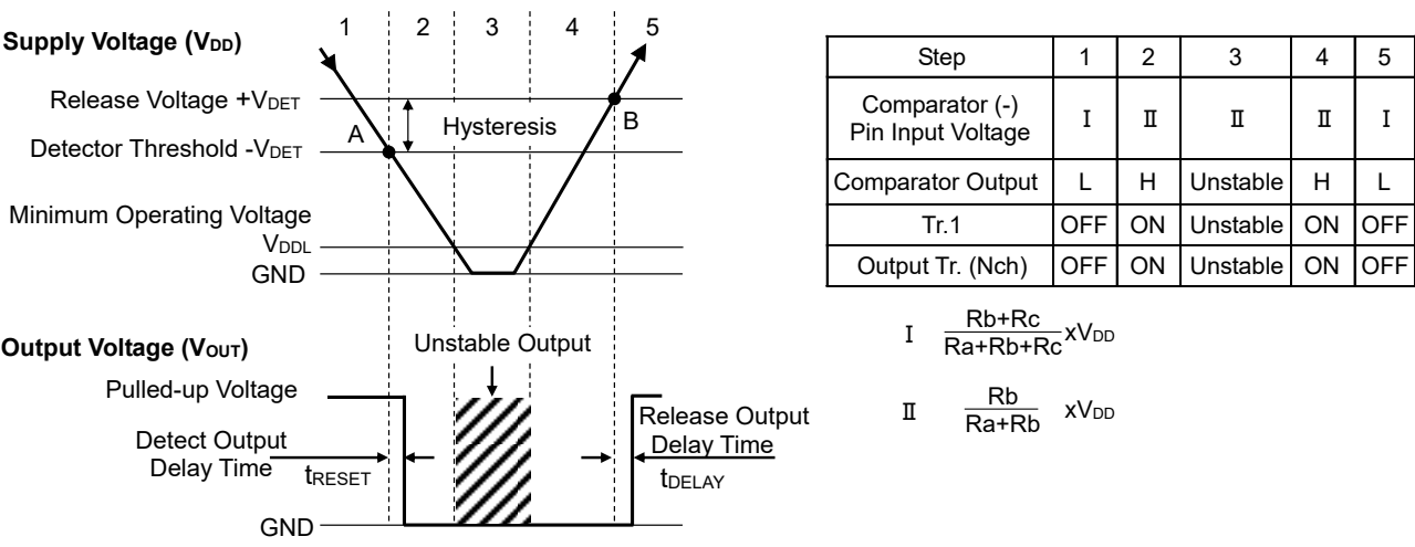
Operation Diagram
