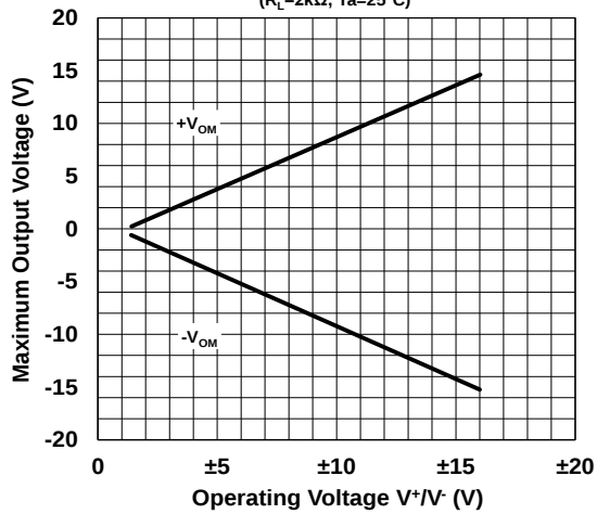
Maximum Output Voltage vs. Operating Voltage ( R_L=2k\Omega , T_a=25^\circ\text{C} )
