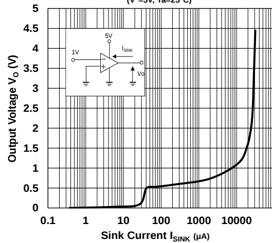
Output Voltage vs. Sink Current ( V^+=5\text{V} , T_a=25^\circ\text{C} )
