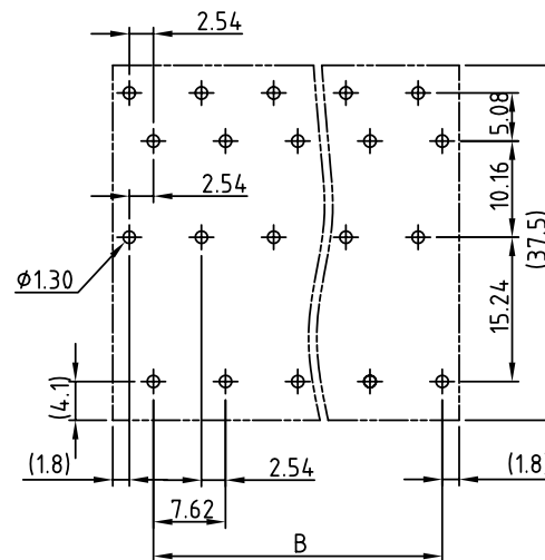
PCB Layout
