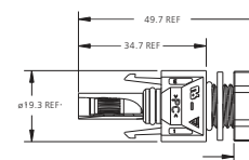
H4 Female PV Panel Connector
