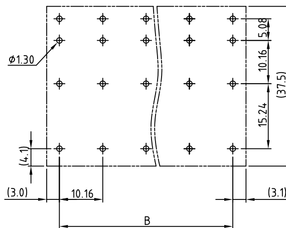
PCB Layout
