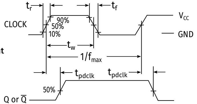
Figure 5: Timing measurements
