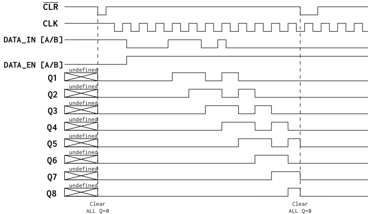
Figure 3: Timing Diagram
