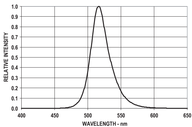
Figure 2. Relative Intensity vs wavelength for HLMP-NM31
