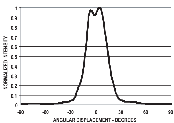
Figure 6. Radiation pattern
