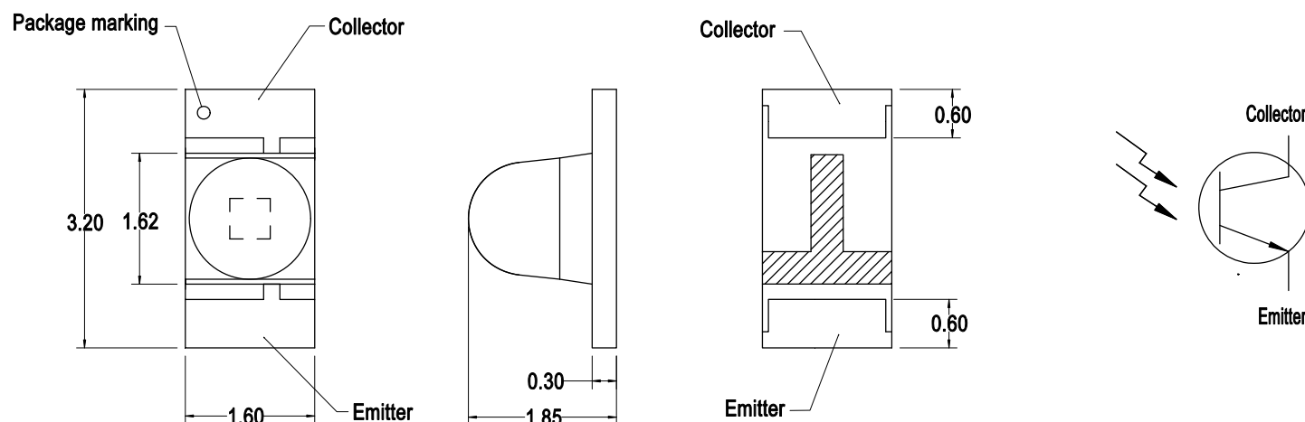
Figure 1: Package Drawing
