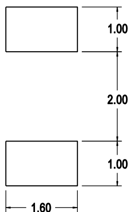
Figure 8: Recommended Soldering Land Pattern
