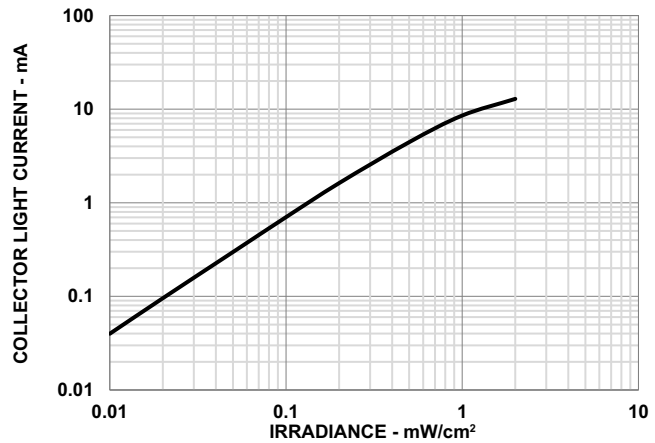
Figure 5: Collector Light Current vs. Irradiance
