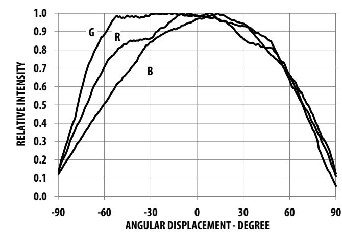
Figure 5: Radiation Pattern
