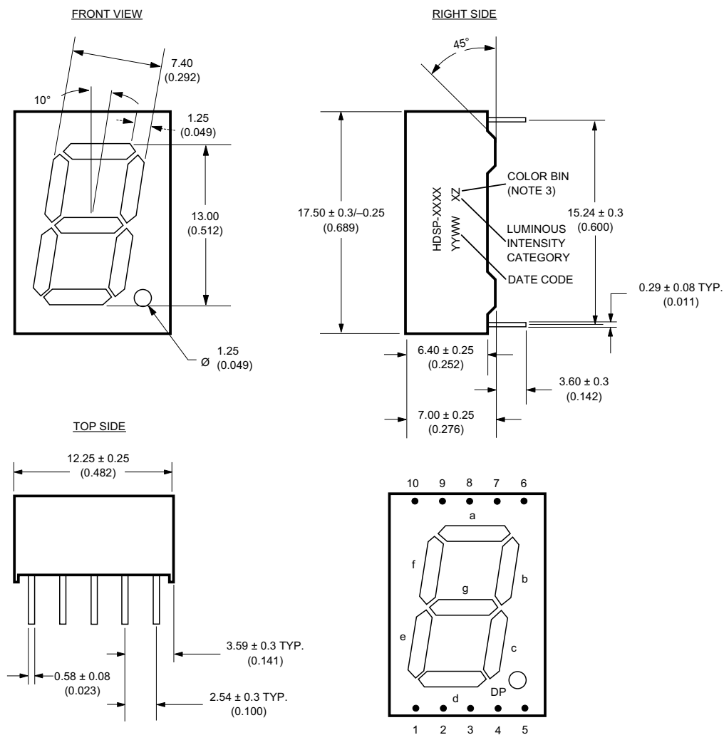
Figure 2: HDSP-561x/563x Series
