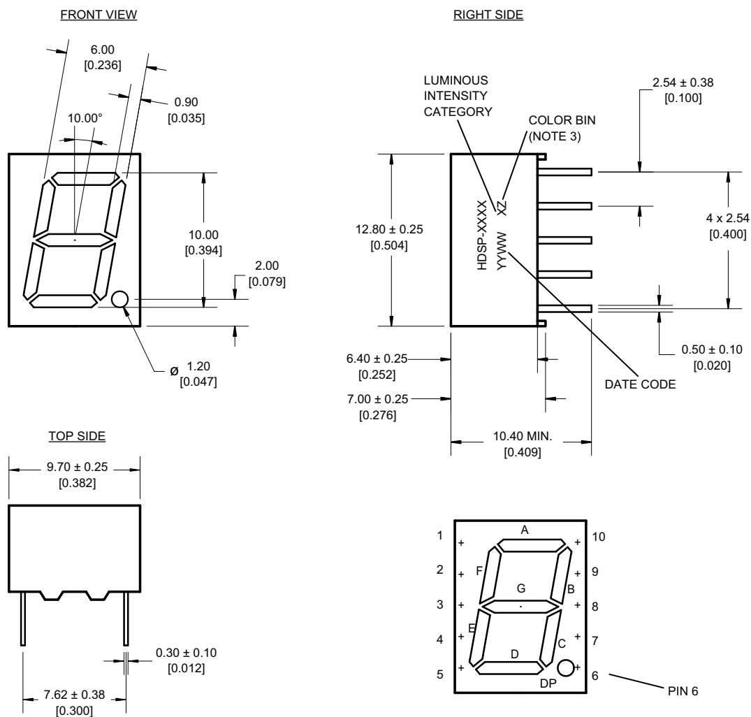
Figure 1: HDSP-301x/303x Series
