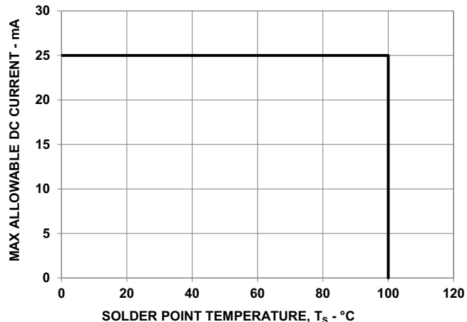
Figure 15: Maximum Forward Current vs. Solder Point Temperature. Derated based on T_{JMAX} = 110^{\circ}\text{C} , R_{\theta J-S} = 80^{\circ}\text{C/W}
