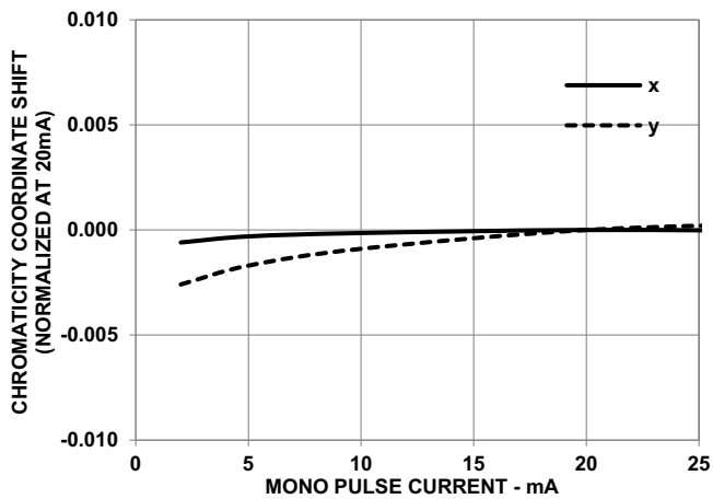
Figure 8: Chromaticity Coordinate Shift vs. Mono Pulse Current (6500K)
