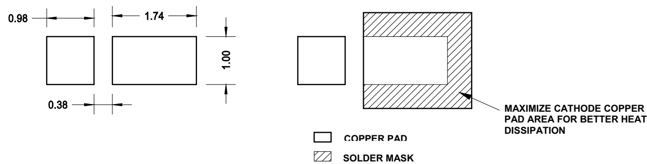
Figure 16: Recommended Soldering Land Pattern
