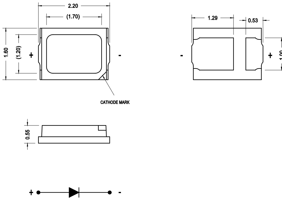
Figure 1: Package Drawing
