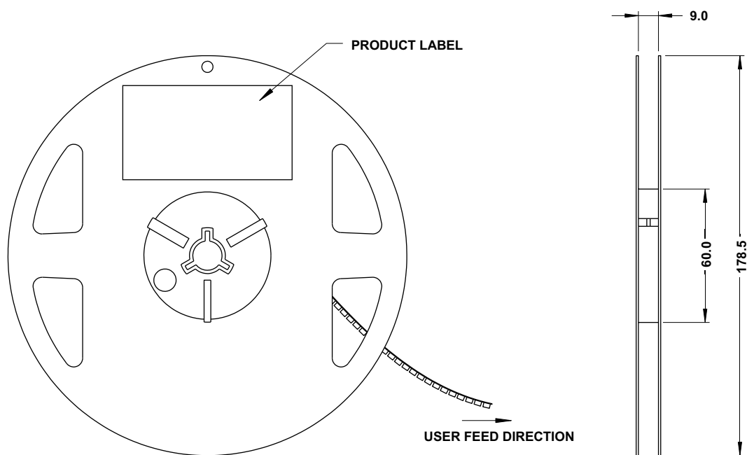
Figure 18: Reel Dimensions
