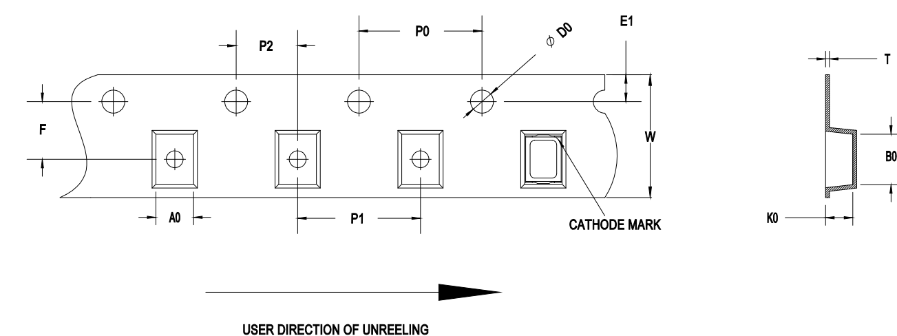
Figure 17: Carrier Tape Dimensions
