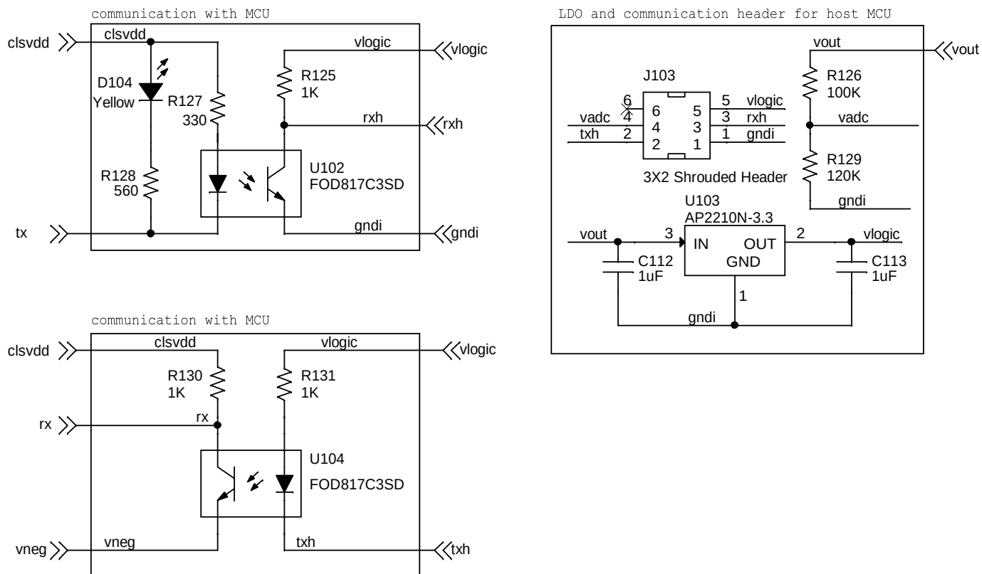
Figure 2.3. Si34071-FW-12V-C8 Schematic: UART Communication (Optional Circuit)
