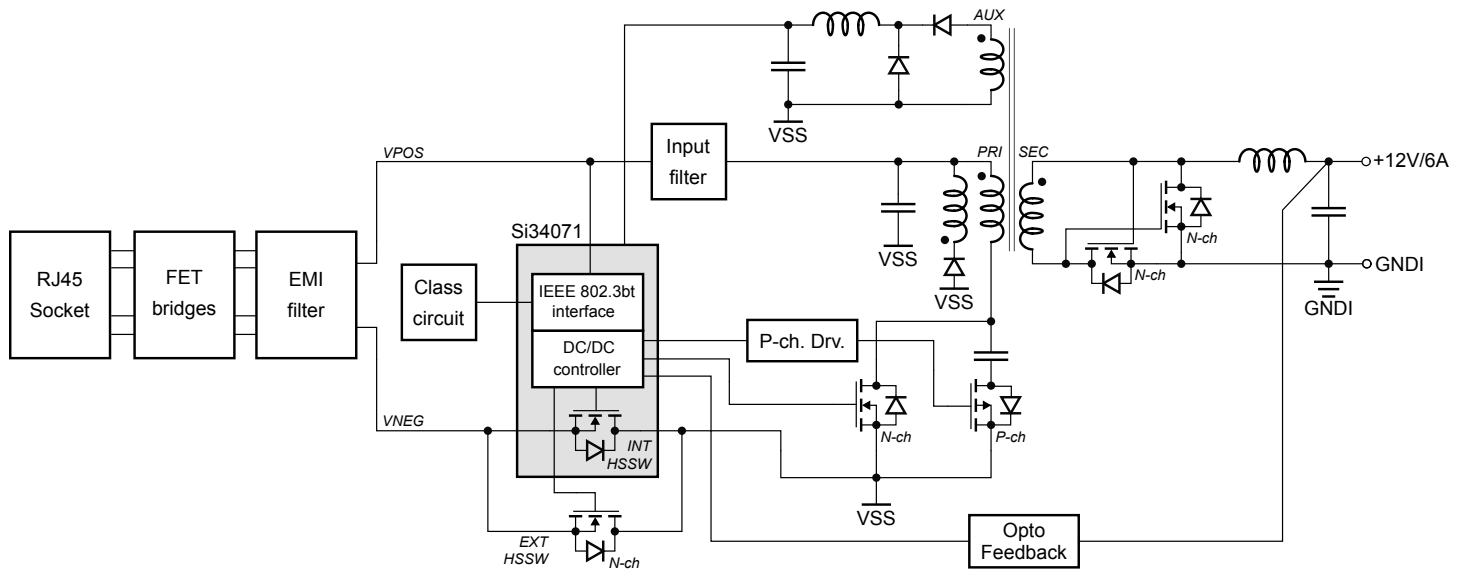
Figure 1.1. Simplified Block Diagram of the Si34071-FW-12V-C8
