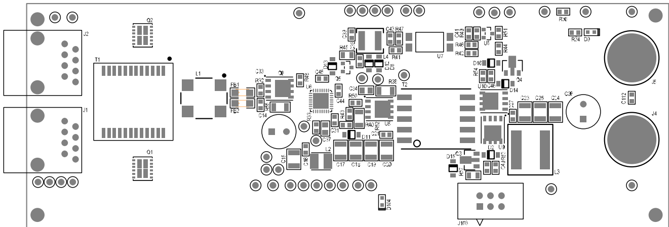
Figure 30. Primary Silkscreen
