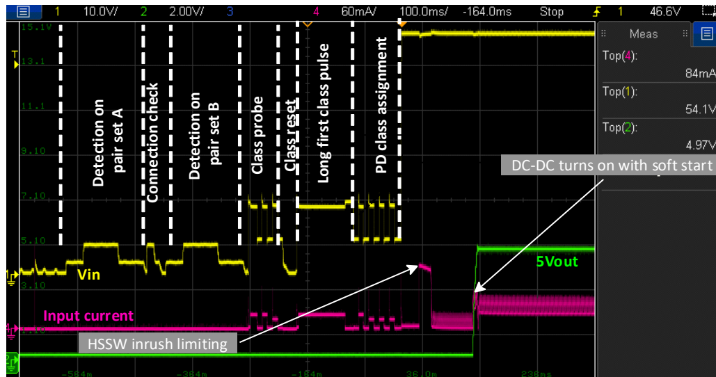
Figure 14. Soft Start Waveforms at No Load Condition
