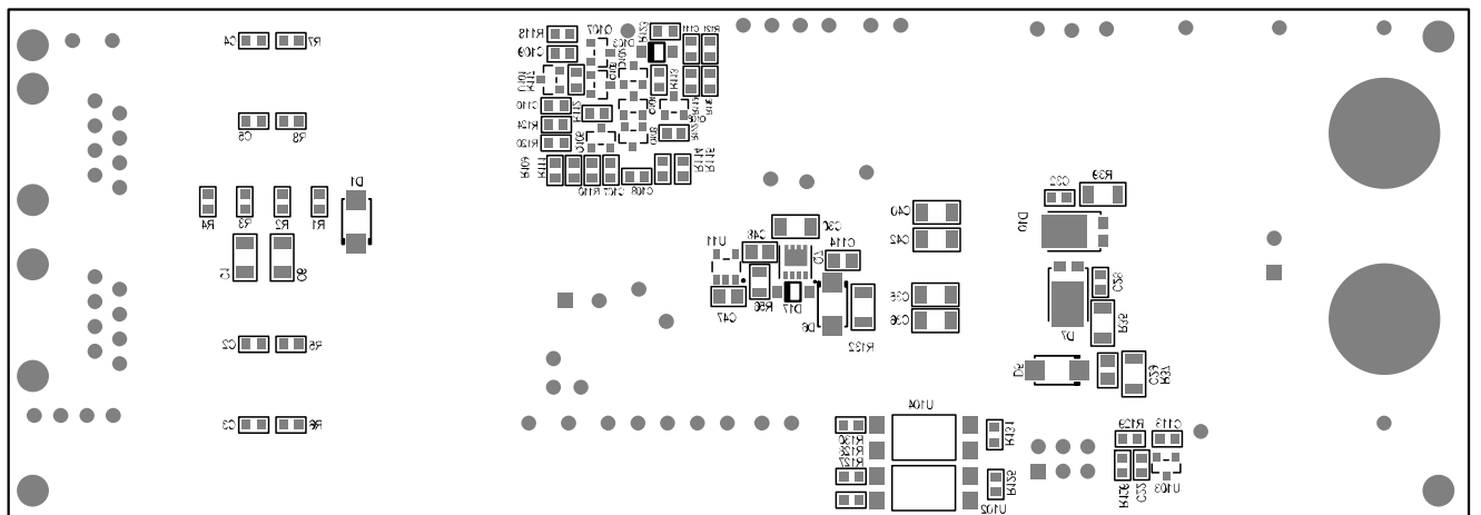
Figure 35. Bottom Silkscreen
