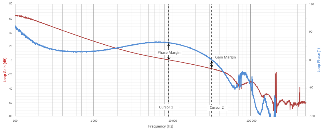
Figure 8. Si34071-FW-5V-C8 EVB Measured Loop-Gain and Phase with 70W Load
