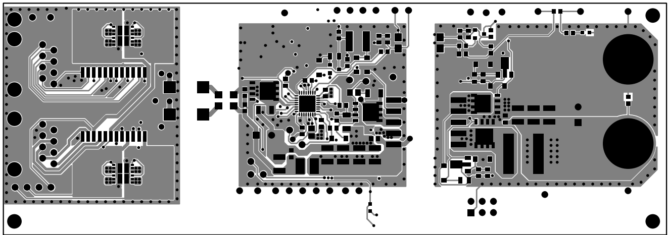
Figure 31. Top Layer
