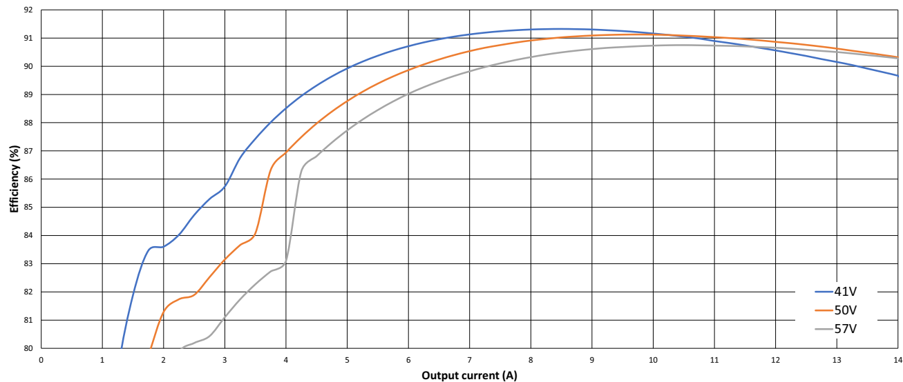
Figure 7. Si34071-FW-5V-C8 EVB End-to-End Conversion Efficiency Chart
