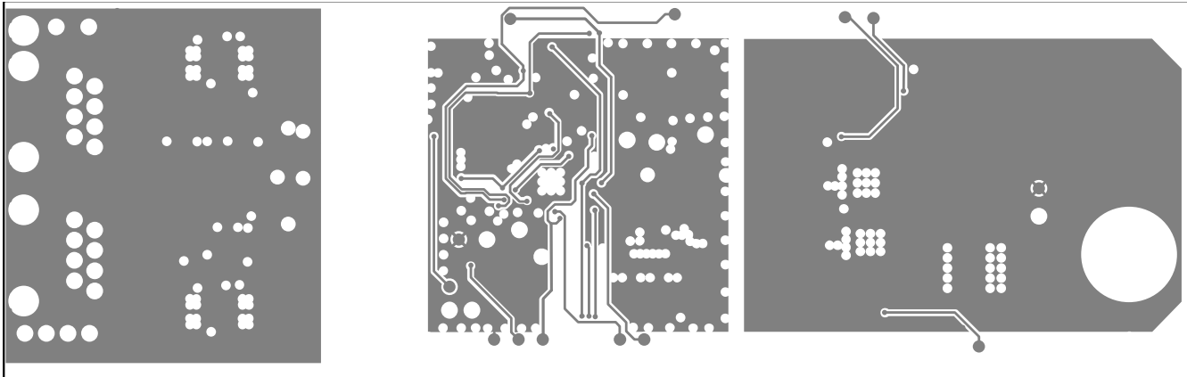
Figure 33. Internal 2 Layer
