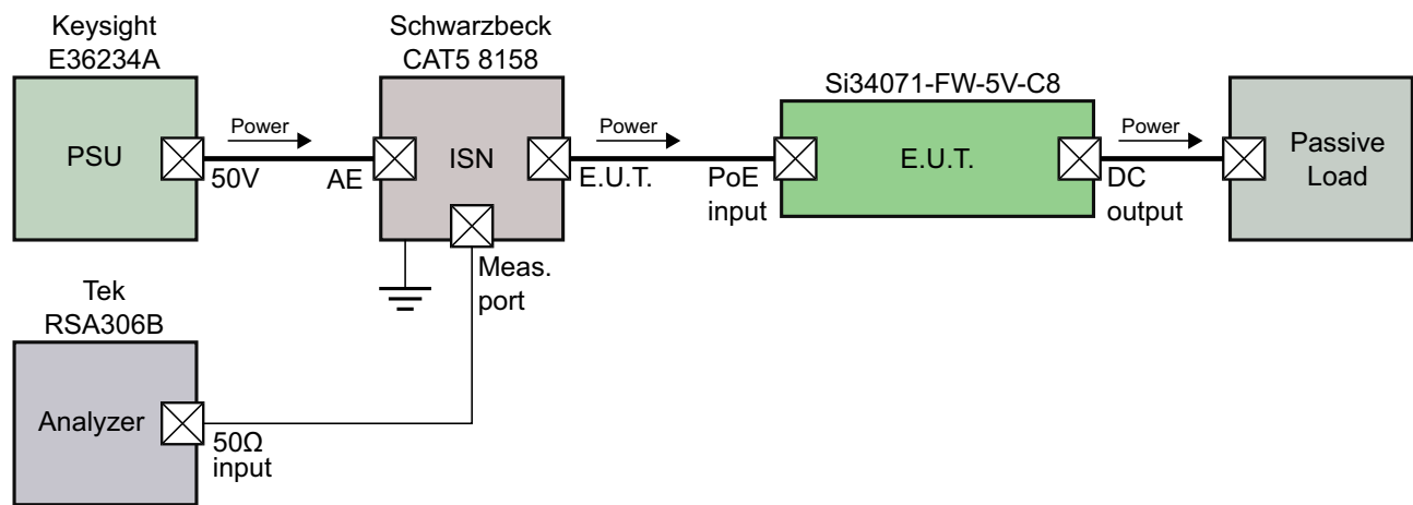
Figure 25. Conducted EMI Measurement Setup
