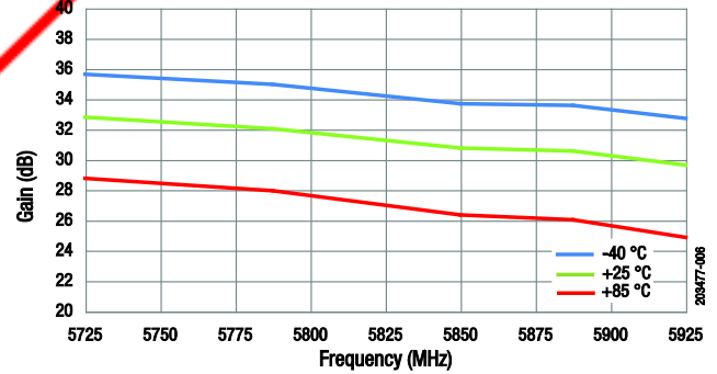
Figure 6. Large Signal Gain @ High Band ( P_{OUT} = +28\text{ dBm, CW} )
