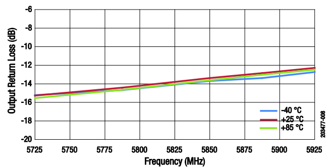
Figure 8. Output Return Loss @ High Band ( P_{IN} = -30\text{ dB} )
