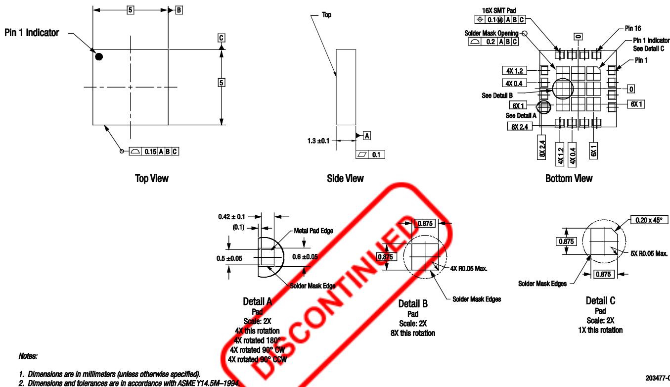
Figure 33. SKY66288-11 Package Dimensions
