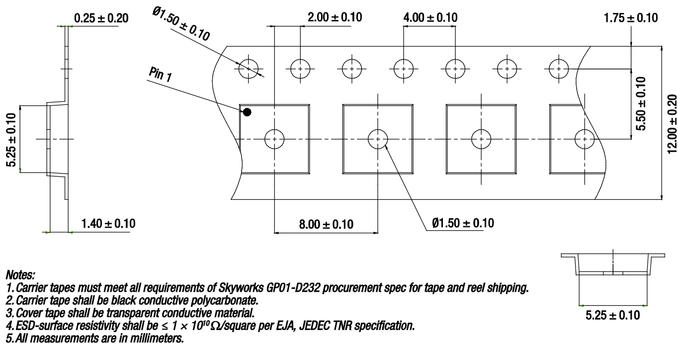
Figure 34. SKY66288-11 Tape and Reel Dimensions
