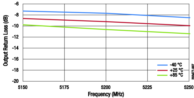
Figure 7. Output Return Loss @ Low Band ( P_{IN} = -30\text{ dB} )
