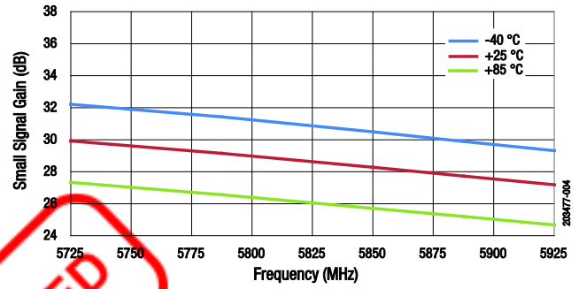
Figure 4. Small Signal Gain @ High Band ( P_{IN} = -30\text{ dB} )
