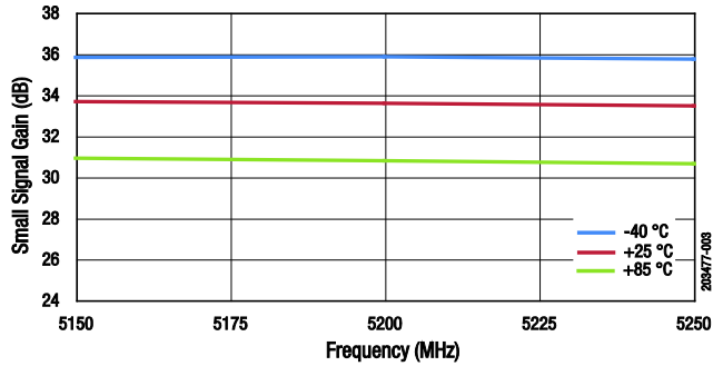
Figure 3. Small Signal Gain @ Low Band ( P_{IN} = -30\text{ dB} )
