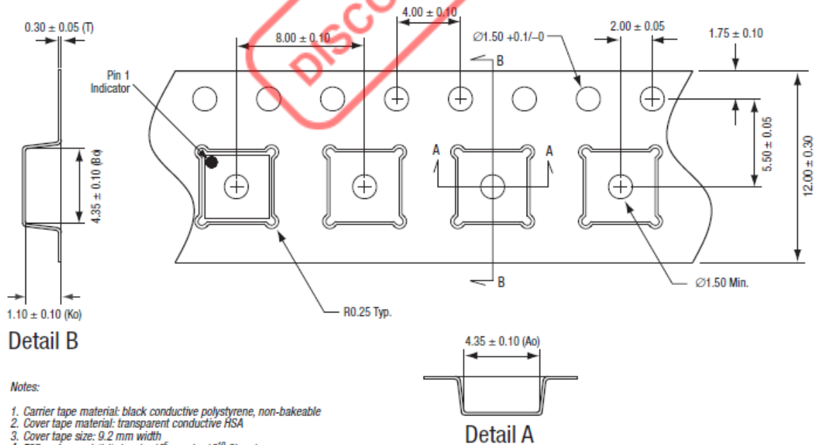
Figure 14. SKY13286-359LF Tape and Reel Dimensions
