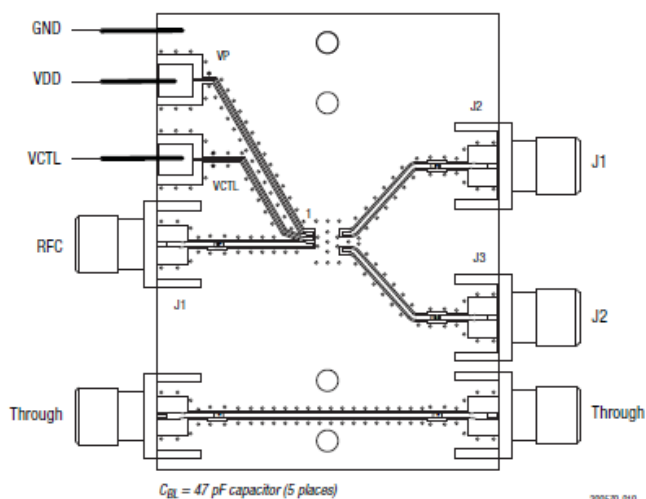
Figure 10. SKY13286-359LF Evaluation Board Assembly Diagram
