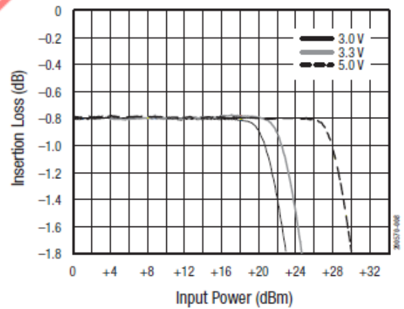
Figure 8. Insertion Loss vs Input Power Over Voltage
