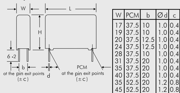
4-pin version
