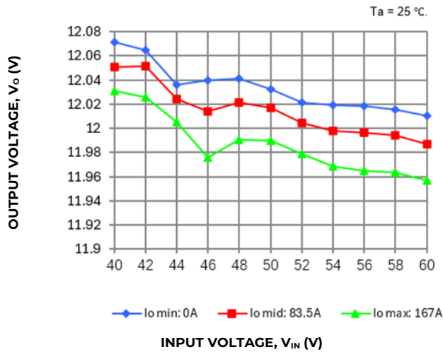
Figure 7. Typical Output Voltage Regulation vs Input Voltage, Without droop
