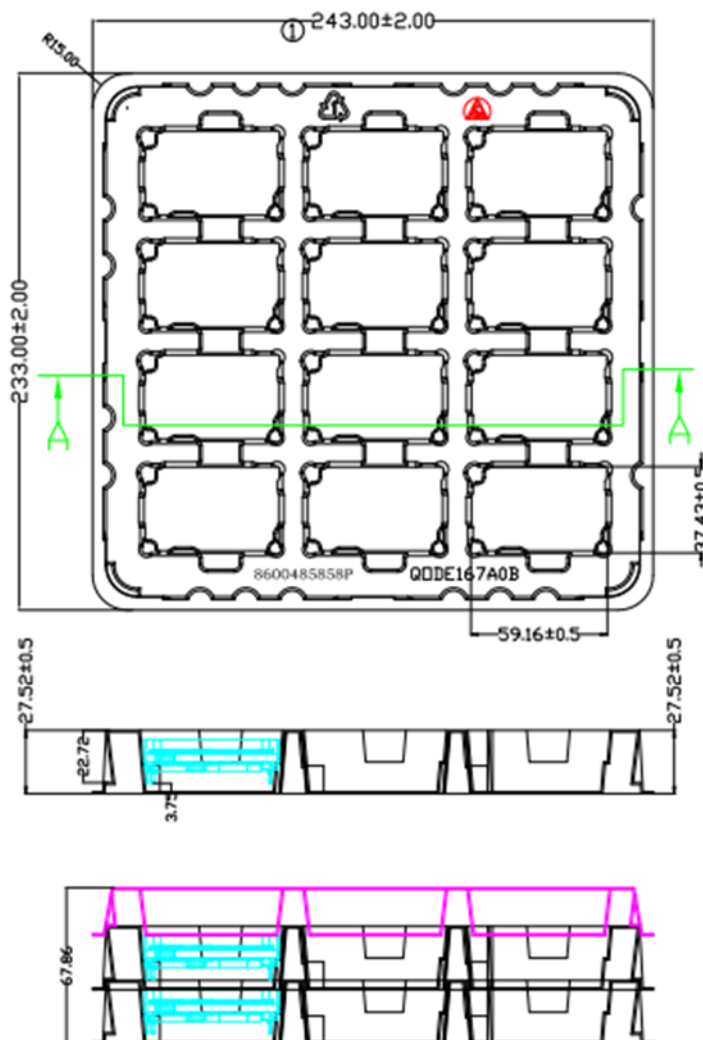
Figure 22. QODE167A0B Packaging Tray
