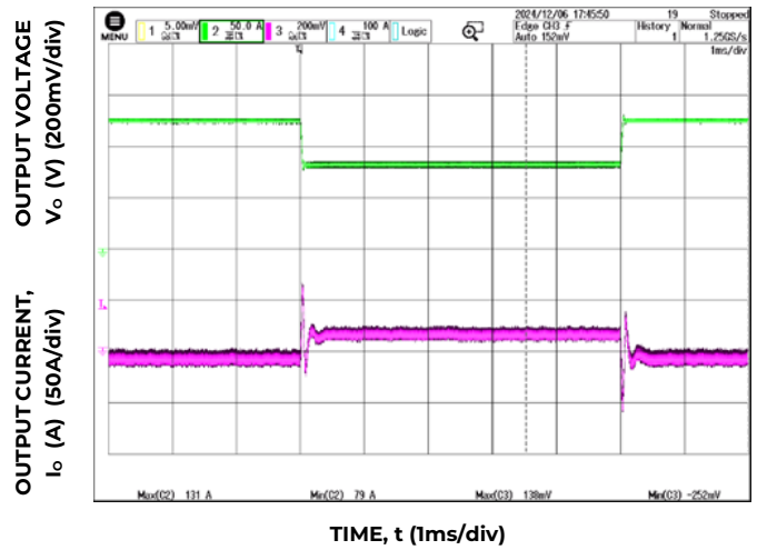
Figure 4. Dynamic Load Response, di_o/dt=1A/\mu s; V_{in}=V_{in,nom} ; T_A=25^\circ C; Load Change from I_o = 50\% to 75\% of I_{o,max} ; C_o = 4200\mu F Ceramic
