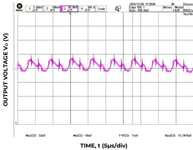
Figure 3. Typical output ripple and noise ( C_o = 350\mu F Ceramic + 3800 \mu F PosCap Oscon, V_{in} = 54 V, I_o = I_{o,max} )
