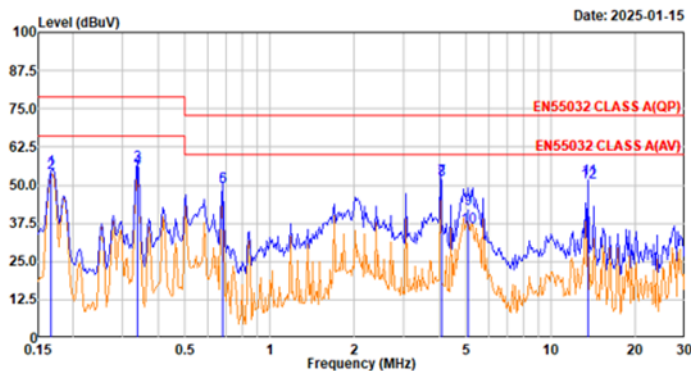
Figure 9. EMI with filter
