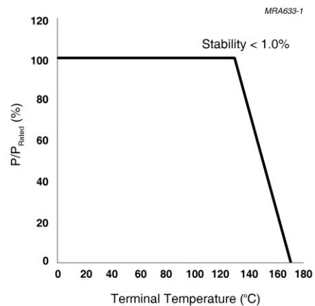
Fig. 6 Stability Performance
