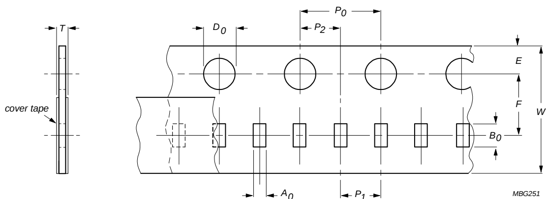
Fig. 14 Paper/PE Tape
