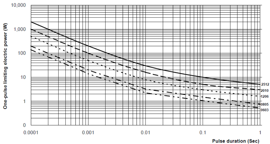
Fig. 13 Maximum permissible peak pulse power as a function of pulse duration
