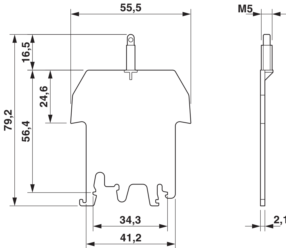
Dimensional drawing
