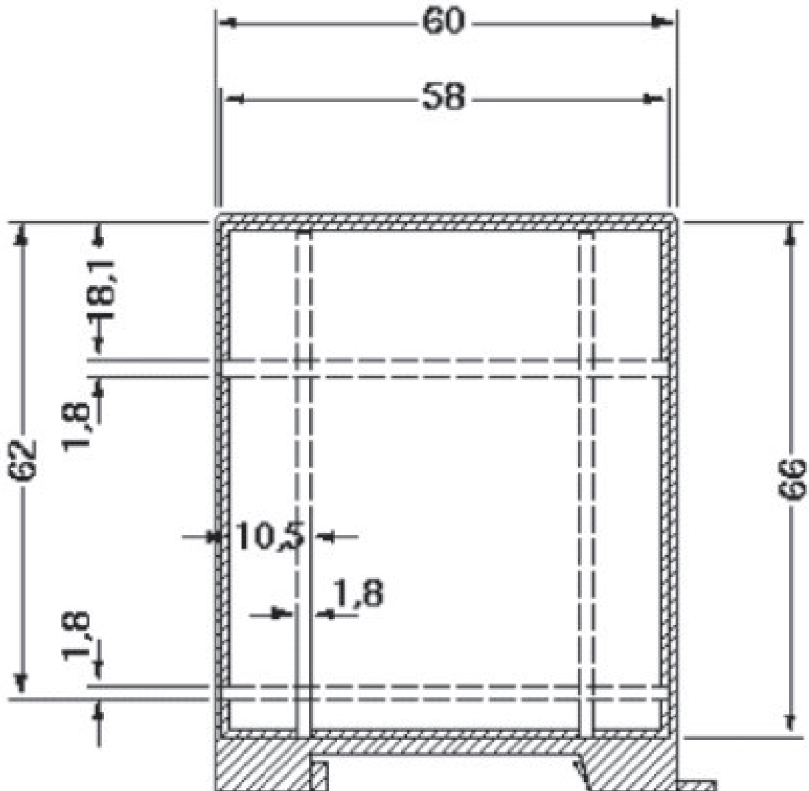
Dimensional drawing
