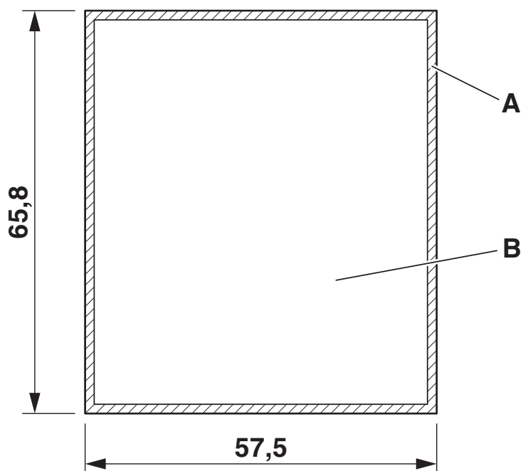
Dimensional drawing
